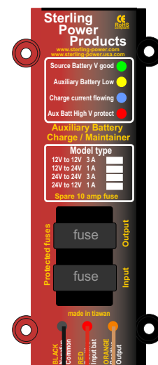
Battery Maintainer Install
